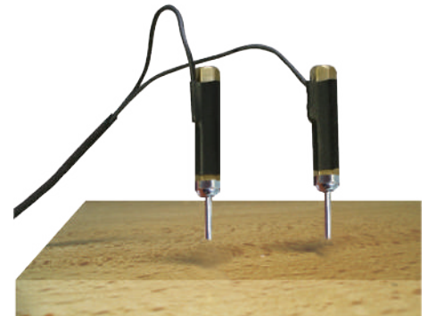
No.7018 Twin Electrodes Probe
